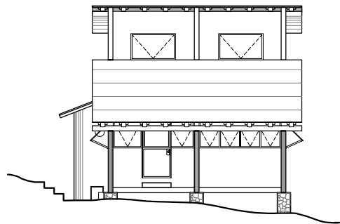
FACHADA PRINCIPAL
