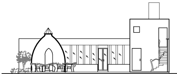
FACHADA PRINCIPAL
